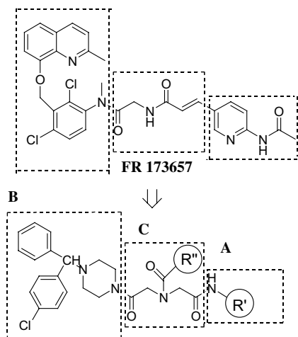
Scheme 1. Design of the iminodiacetic acid triamide derivatives based on FR 173657.
