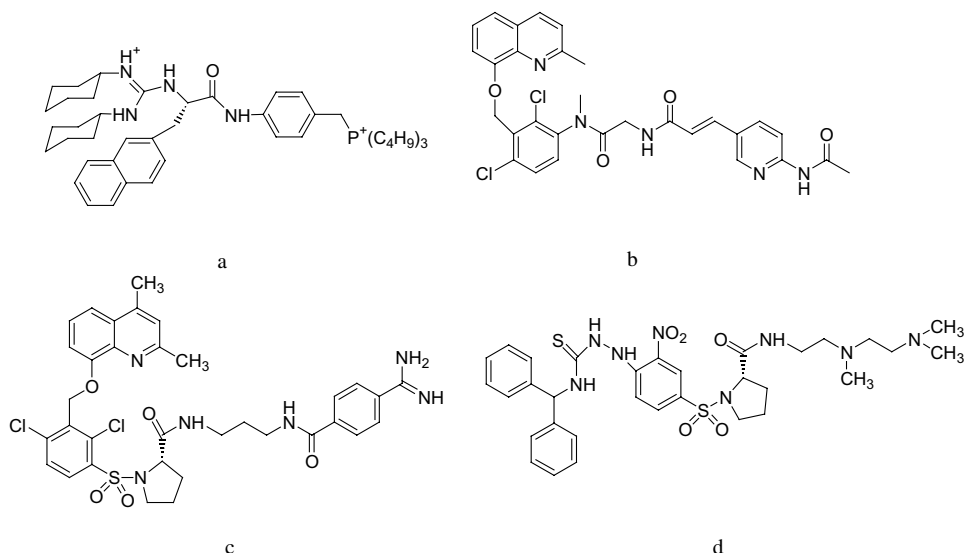
Figure 1. The structure of Win 64338 (a), FR 173657 (b), LF 16-0687 (c), and Bradyzide (d).
