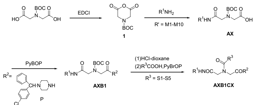
Scheme 2. Solution-phase combinatorial synthesis route using the iminodiacetic anhydride template.
